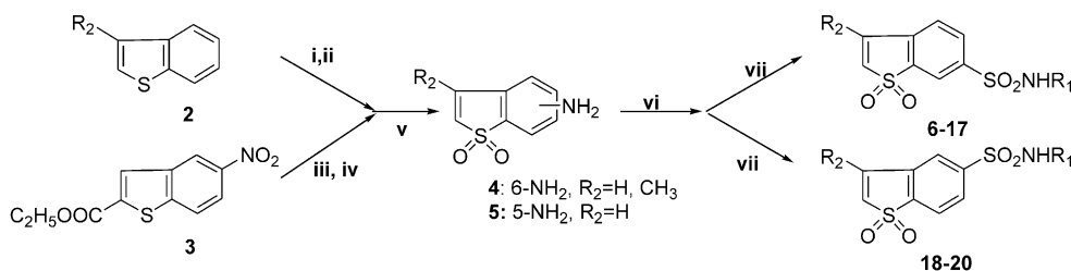
Scheme 1. (i) Acetic acid, \text{H}_2\text{O}_2 30% (v/v), reflux, 30 min; (ii) nitric acid 100%; (iii) NaOH, Ethyl alcohol/water 50%; Cu/Quinolin 200 °C; (iv) MCPBA; (v) Fe/ \text{NH}_4\text{Cl} , ethanol/ \text{H}_2\text{O} 50% (v/v); (vi) \text{NaNO}_2 , HCl (ac); \text{SO}_2 /CuCl, Acetic acid; (vii) \text{NH}_2\text{R} , dioxane.
